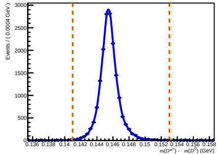
Passed DiF (after RICH1) ( 0 < nTracks < 200 , 3.6 < \eta < 5.0 , 15600 < p < 27000 )
