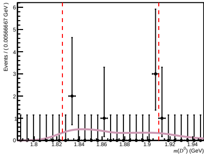
Passed ( 200 < n\text{Tracks} < 600 , 3.6 < \eta < 5.0 , 10000 < p < 15600 )
