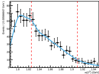
Total ( 200 < n_{\text{Tracks}} < 600 , 3.6 < \eta < 5.0 , 27000 < p < 60000 )
