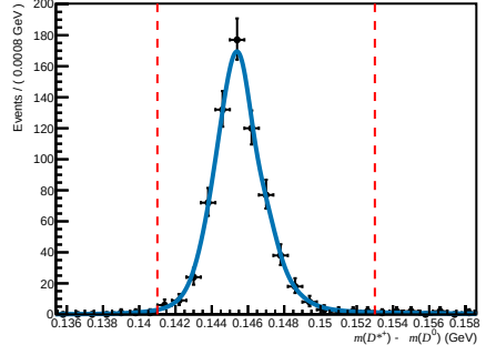
Total ( 0 < n\text{Tracks} < 200 , 1.7 < \eta < 3.6 , 6000 < p < 10000 )
