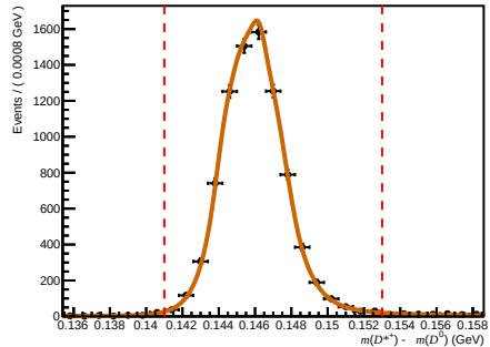
Failed ( 0 < n\text{Tracks} < 200 , 1.7 < \eta < 3.6 , 6000 < p < 10000 )
