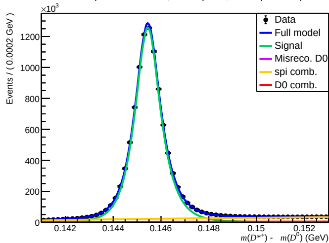
Failed ( 0 < n\text{Tracks} < 200 , 1.7 < \eta < 3.6 , 6000 < p < 10000 )
