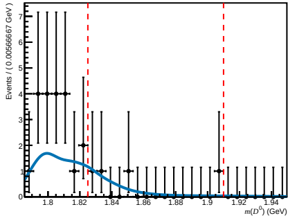
Failed ( 0 < nTracks < 200 , 3.6 < \eta < 5.0 , 27000 < p < 60000 )
