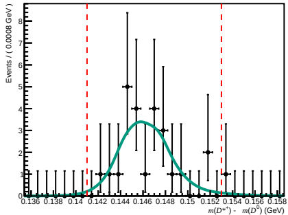
Failed ( 200 < n\text{Tracks} < 600 , 1.7 < \eta < 3.6 , 3000 < p < 6000 )
