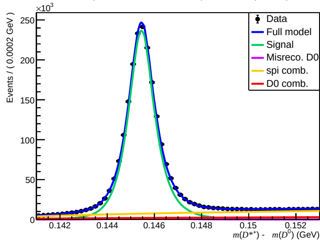
Failed (200 < nTracks < 600, 1.7 < \eta < 3.6, 3000 < p < 6000)
