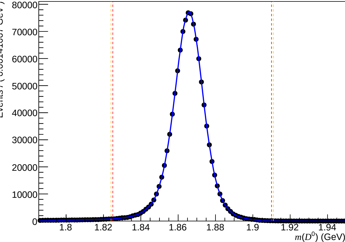
Failed non-DiF ( 200 < nTracks < 600 , 1.7 < \eta < 3.6 , 6000 < p < 10000 )
