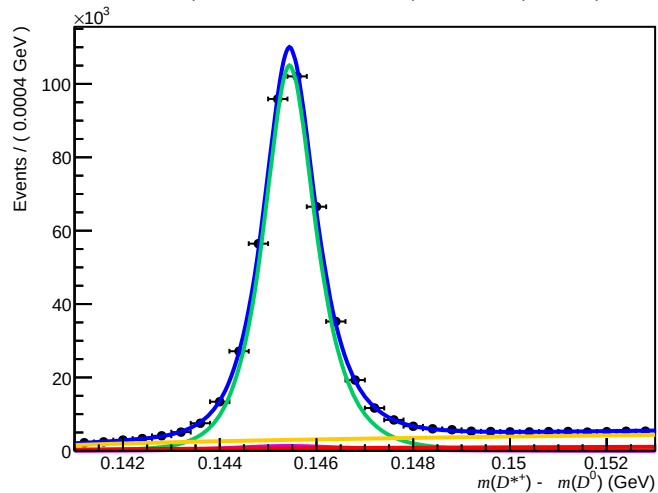
Passed ( 200 < n\text{Tracks} < 600 , 1.7 < \eta < 3.6 , 6000 < p < 10000 )
