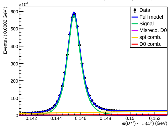
Failed ( 200 < n\text{Tracks} < 600 , 1.7 < \eta < 3.6 , 6000 < p < 10000 )
