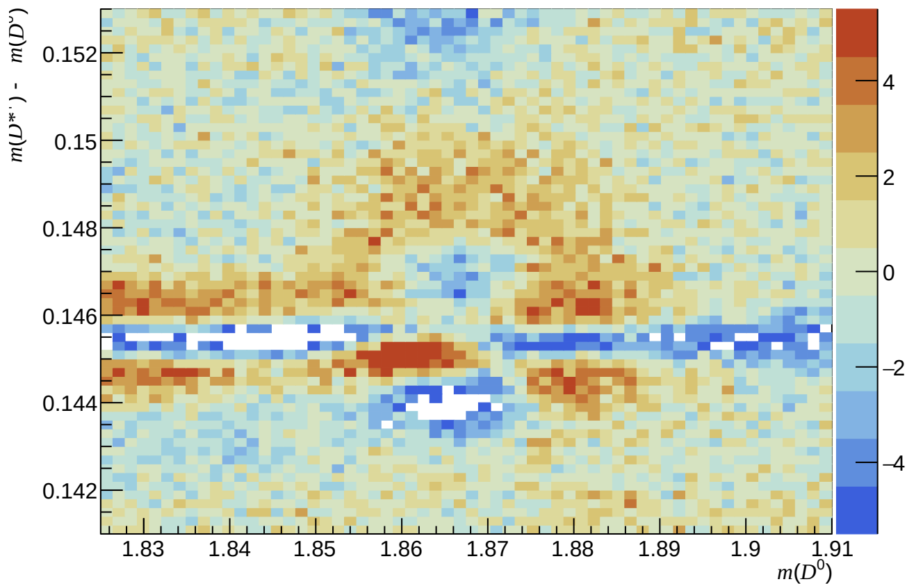
Failed ( 0 < nTracks < 200 , 1.7 < \eta < 3.6 , 10000 < p < 15600 )
