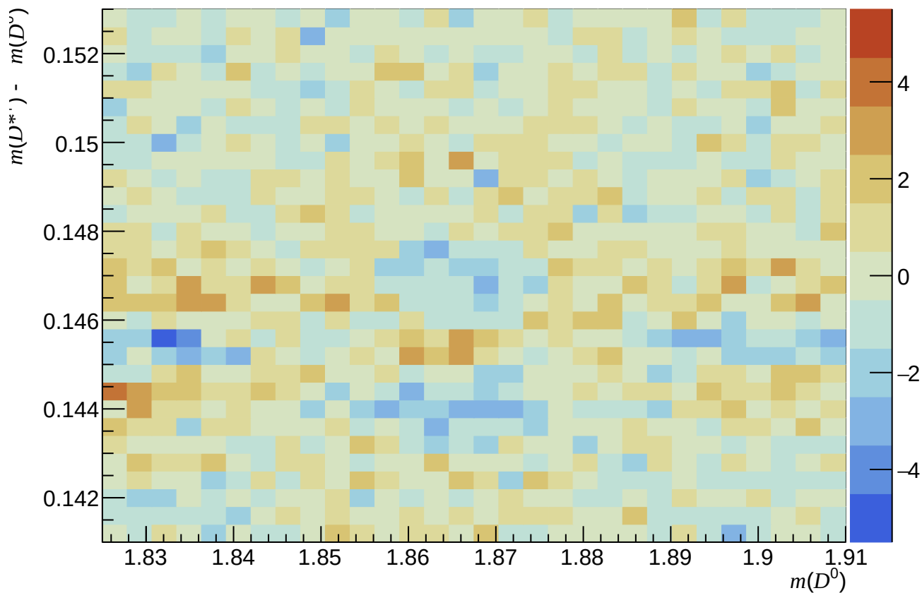
Passed ( 0 < nTracks < 200 , 1.7 < \eta < 3.6 , 10000 < p < 15600 )
