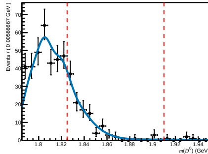
Total ( 0 < nTracks < 200 , 3.6 < \eta < 5.0 , 10000 < p < 15600 )
