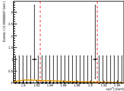
Passed ( 0 < nTracks < 200 , 3.6 < \eta < 5.0 , 15600 < p < 27000 )
