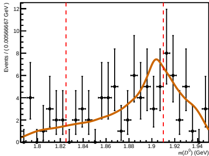
Passed ( 0 < n\text{Tracks} < 200 , 3.6 < \eta < 5.0 , 27000 < p < 60000 )
