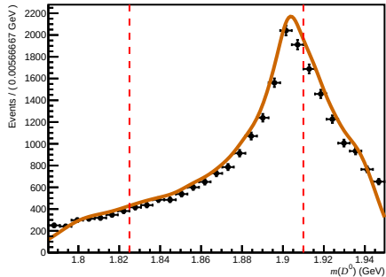
Failed ( 0 < n\text{Tracks} < 200 , 3.6 < \eta < 5.0 , 27000 < p < 60000 )
