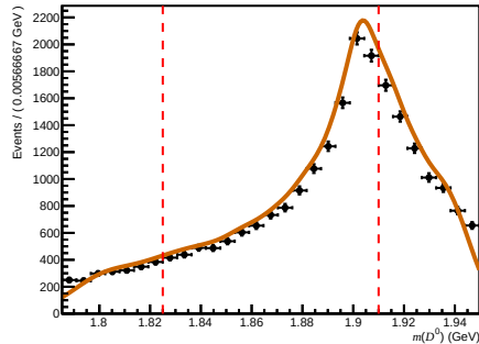
Total ( 0 < n\text{Tracks} < 200 , 3.6 < \eta < 5.0 , 27000 < p < 60000 )
