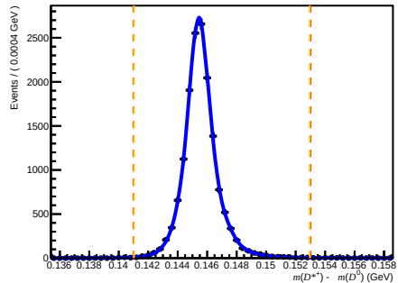
Passed DiF (after RICH1) ( 0 < nTracks < 200 , 3.6 < \eta < 5.0 , 27000 < p < 60000 )
