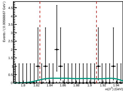
Passed ( 200 < nTracks < 600 , 1.7 < \eta < 3.6 , 3000 < p < 6000 )
