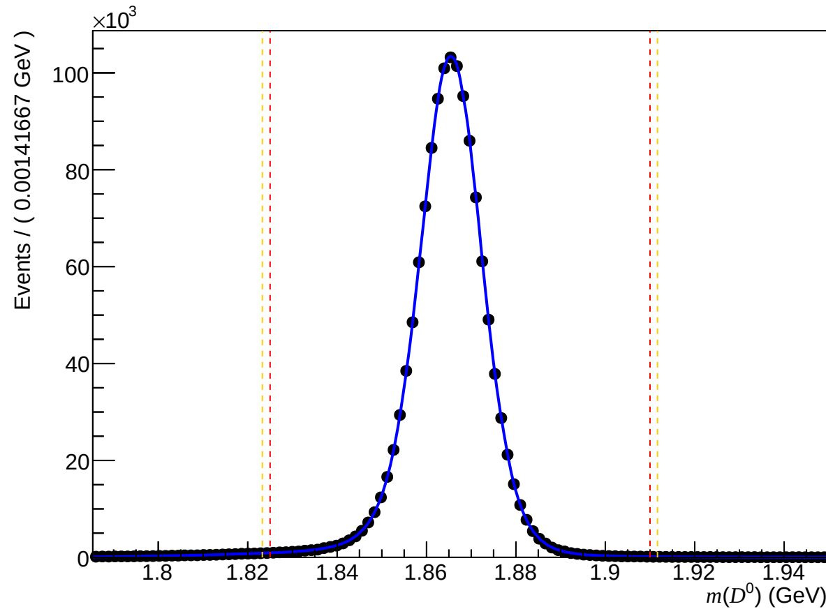
Failed non-DiF ( 200 < nTracks < 600 , 1.7 < \eta < 3.6 , 10000 < p < 15600 )
