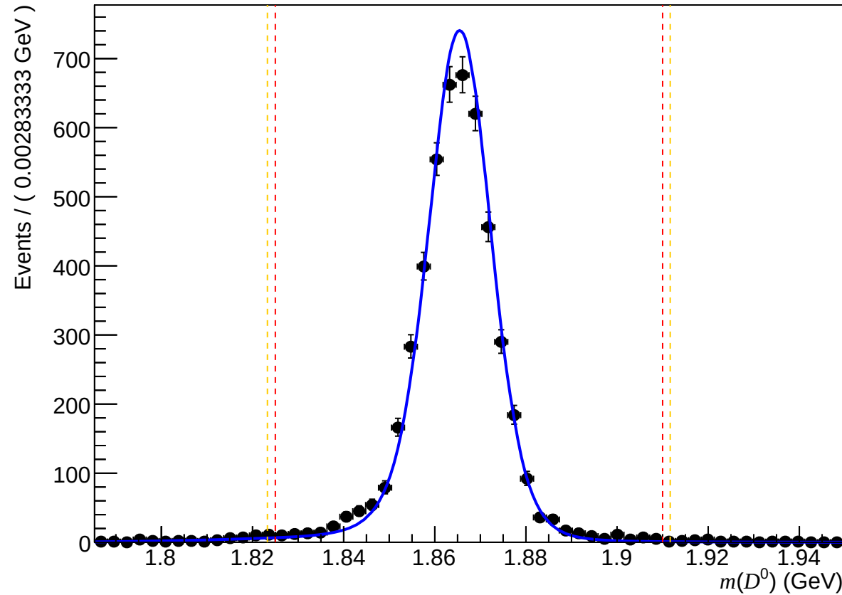
Passed non-DiF ( 200 < nTracks < 600 , 1.7 < \eta < 3.6 , 10000 < p < 15600 )
