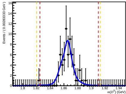
Passed DiF (after RICH1) ( 200 < n\text{Tracks} < 600 , 3.6 < \eta < 5.0 , 3000 < p < 6000 )
