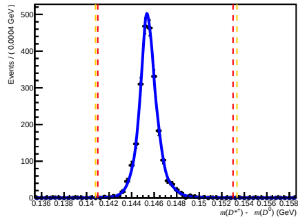
Failed Df ( 0 < nTracks < 200 , 1.7 < \eta < 3.6 , 60000 < p < 100000 )
