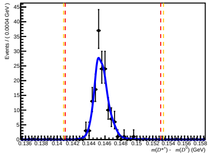
Passed Df (after RICH1) ( 0 < nTracks < 200 , 1.7 < \eta < 3.6 , 60000 < p < 100000 )
