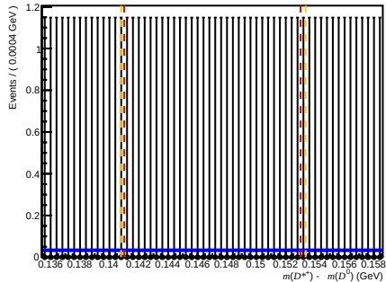
Passed Df (before RICH1) ( 0 < nTracks < 200 , 1.7 < \eta < 3.6 , 60000 < p < 100000 )
