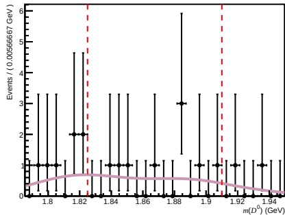
Total ( 200 < nTracks < 600 , 1.7 < \eta < 3.6 , 3000 < p < 6000 )
