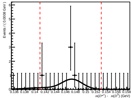
Total ( 200 < nTracks < 600 , 1.7 < \eta < 3.6 , 6000 < p < 10000 )
