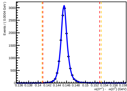
Failed DiF ( 200 < n_{\text{Tracks}} < 600 , 1.7 < \eta < 3.6 , 15600 < p < 27000 )
