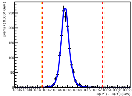
Passed DiF (after RICH1) ( 200 < n_{\text{Tracks}} < 600 , 1.7 < \eta < 3.6 , 15600 < p < 27000 )
