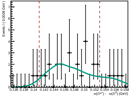
Passed ( 200 < n\text{Tracks} < 600 , 1.7 < \eta < 3.6 , 60000 < p < 100000 )
