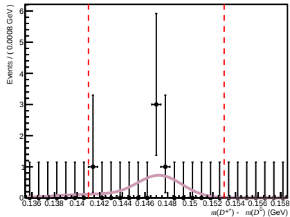
Total ( 200 < nTracks < 600 , 3.6 < \eta < 5.0 , 6000 < p < 10000 )
