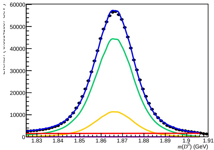
Failed ( 200 < n\text{Tracks} < 600 , 3.6 < \eta < 5.0 , 10000 < p < 15600 )
