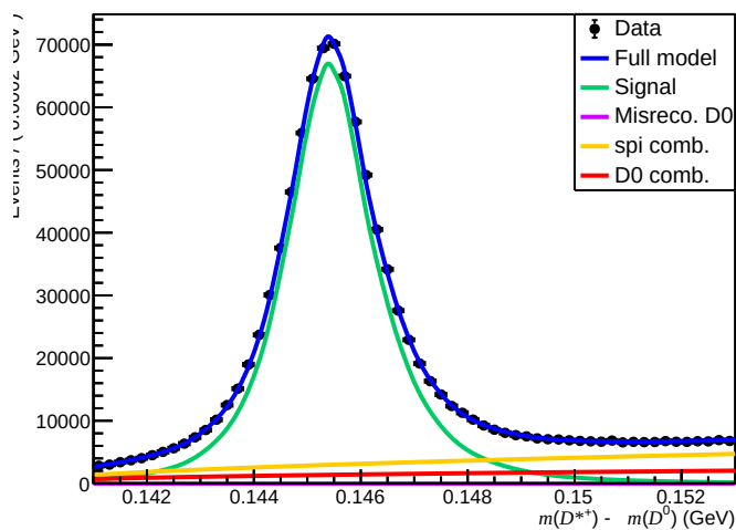
Failed ( 200 < n\text{Tracks} < 600 , 3.6 < \eta < 5.0 , 10000 < p < 15600 )
