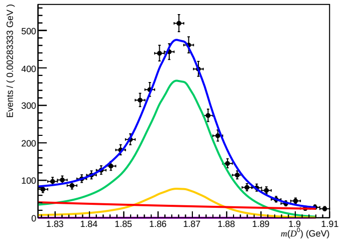
Failed ( 200 < n\text{Tracks} < 600 , 3.6 < \eta < 5.0 , 10000 < p < 15600 )
