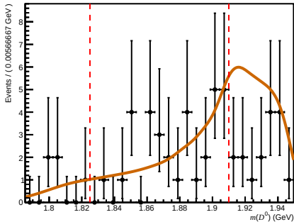
Passed ( 200 < n\text{Tracks} < 600 , 3.6 < \eta < 5.0 , 27000 < p < 60000 )
