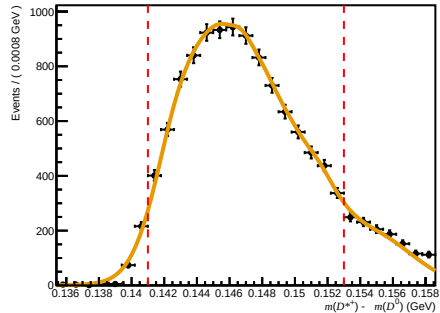
Failed ( 200 < n\text{Tracks} < 600 , 3.6 < \eta < 5.0 , 27000 < p < 60000 )
