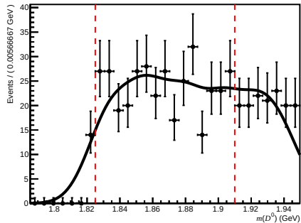
Failed ( 200 < n\text{Tracks} < 600 , 3.6 < \eta < 5.0 , 60000 < p < 100000 )
