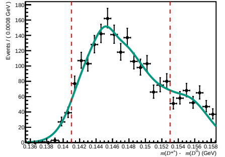
Total ( 200 < nTracks < 600 , 3.6 < \eta < 5.0 , 60000 < p < 100000 )
