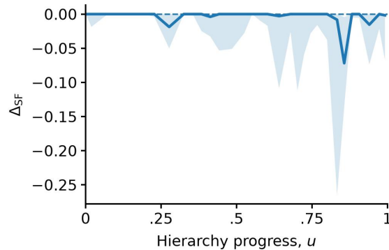
Feshbach gain
