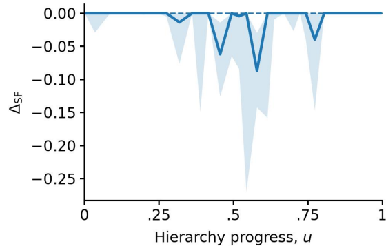
Feshbach gain
