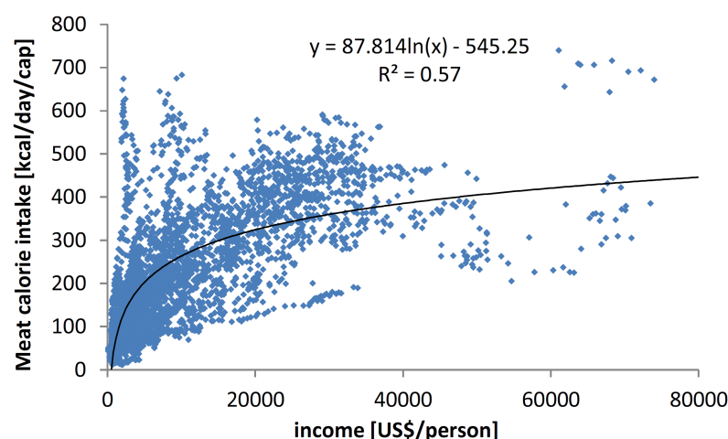
Figure 11.3: Time-series and cross-country data on meat calorie intake and income (1980-2009, source: World Bank (2013) [?] for income and Food and Agriculture Organization of the United Nations (2013) [?] for calorie intake)
