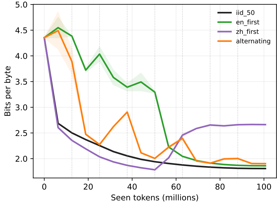
ZH order effect
