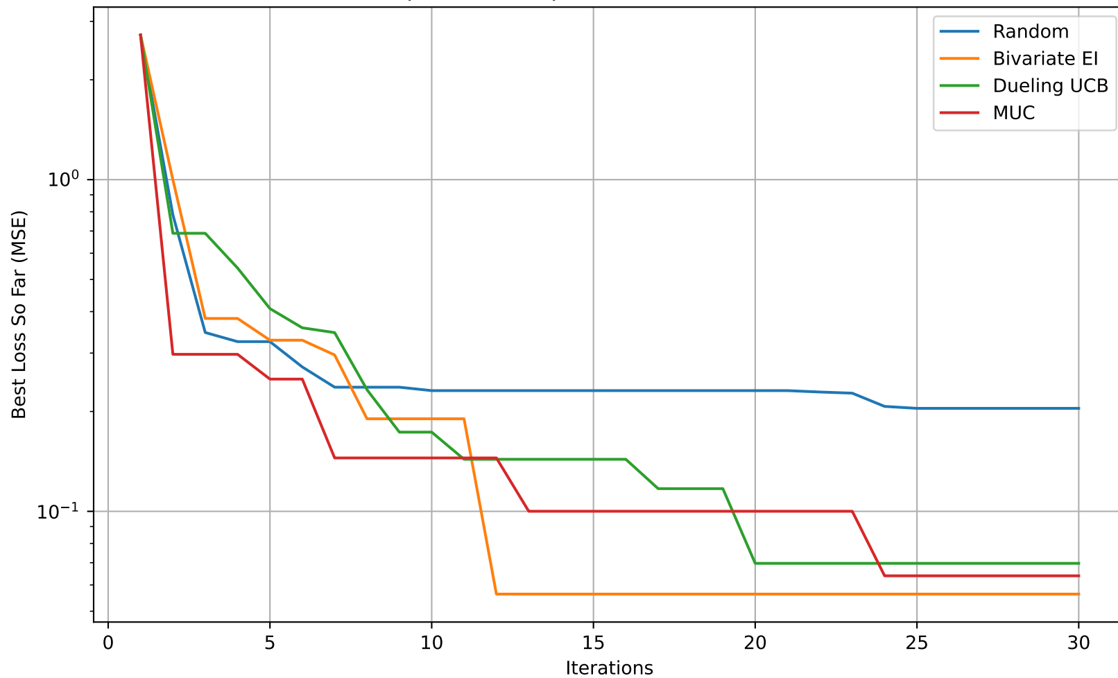
Acquisition Comparison (Kernel: Matern52)
