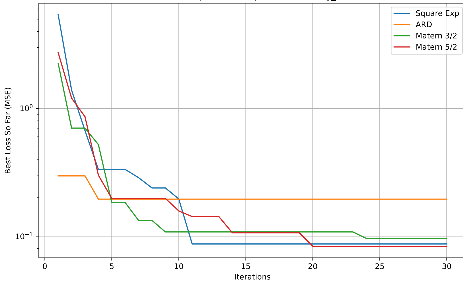
Kernel Comparison (Acquisition: Dueling_UCB)
