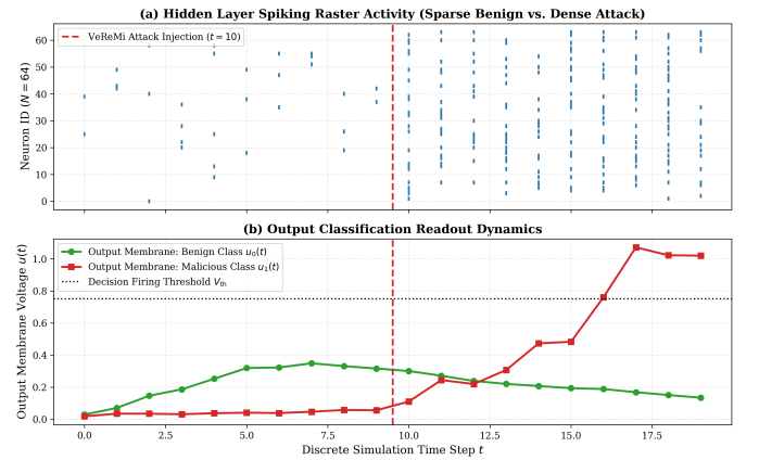
Fig. 8. (a) Spiking raster plot of 64 hidden neurons under sparse benign telemetry ( t < 10 ) transitioning to dense firing during VeReMi attack injection ( t \geq 10 ). (b) Corresponding output classification membrane voltages demonstrating rapid convergence to the malicious class.
