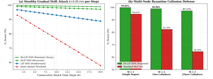
Fig. 10. (a) F_1 -score degradation under stealthy gradual drift attacks ( +0.05 m/s ramp per step) showing KA-LIF resilience due to dynamic membrane leak acceleration. (b) Multi-node Byzantine collision defense against M = 1, 2, 3 colluding rogue vehicles.
