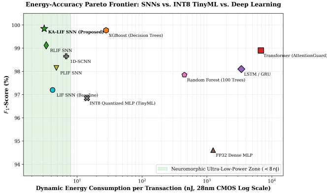
Fig. 9. Energy-Accuracy Pareto frontier on 28nm CMOS silicon. SNNs occupy the ultra-low-power region ( < 8 nJ), outperforming INT8 quantized MLPs (14.2 nJ) and heavy Transformer/LSTM architectures ( > 3,000 nJ).
