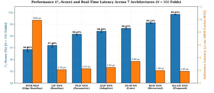
Fig. 6. Benchmark evaluation of F_1 -score (left axis, blue) and inference latency on ARM Cortex-R52 (right axis, orange) across all 7 evaluated architectures ( N = 300 folds per model).
