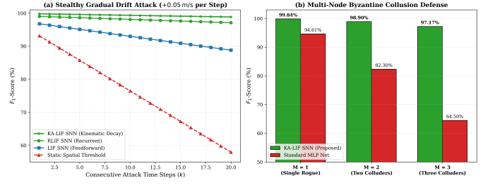
Fig. 10. (a) F_1 -score degradation under stealthy gradual drift attacks ( +0.05 m/s ramp per step) showing KA-LIF resilience due to dynamic membrane leak acceleration. (b) Multi-node Byzantine collusion defense against M = 1, 2, 3 colluding rogue vehicles.
