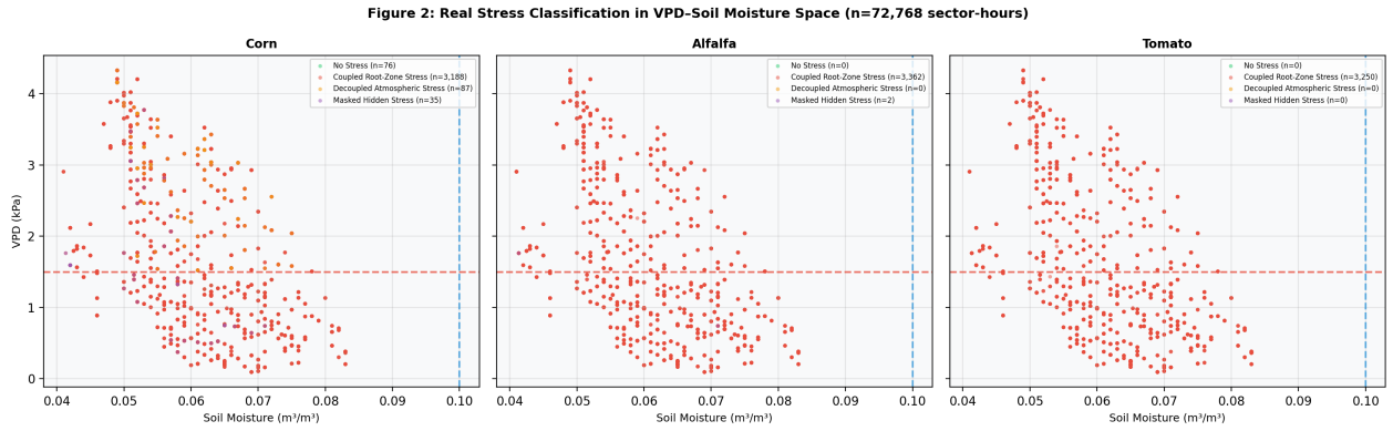
Figure 2: Stress classification in VPD–Soil Moisture space for the three active crop fields. Each point represents a sector-hour observation coloured by its assigned stress category. Red dashed lines mark the VPD = 1.5 kPa atmospheric threshold; blue dashed lines mark the RAW soil moisture boundary. Points in the upper-left quadrant (high VPD, adequate soil moisture) correspond to decoupled atmospheric stress events that would trigger false positive irrigation responses in a thermal-only scheduling system.
