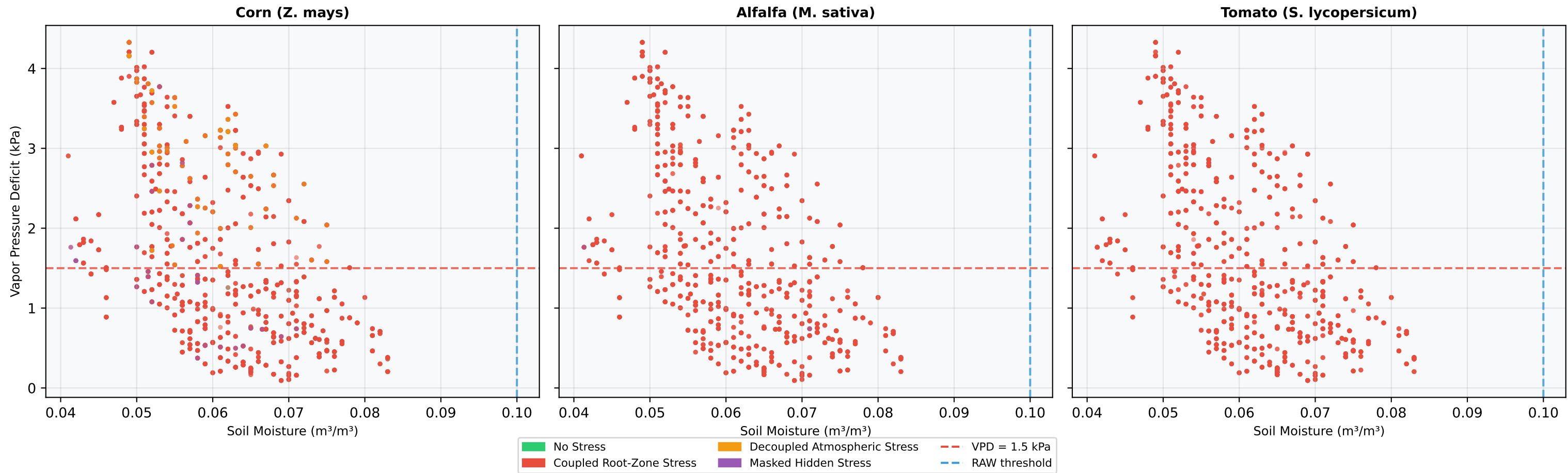
Figure 2: Stress Classification in VPD-Soil Moisture Space by Crop Type
