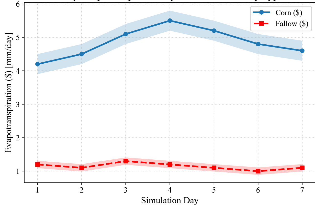
7-Day Evapotranspiration Dynamics Across Crop Types
