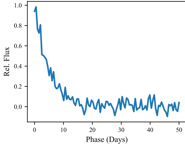
Kilonova Candidate
