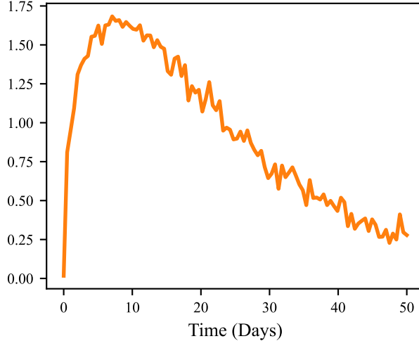
TDE Candidate
