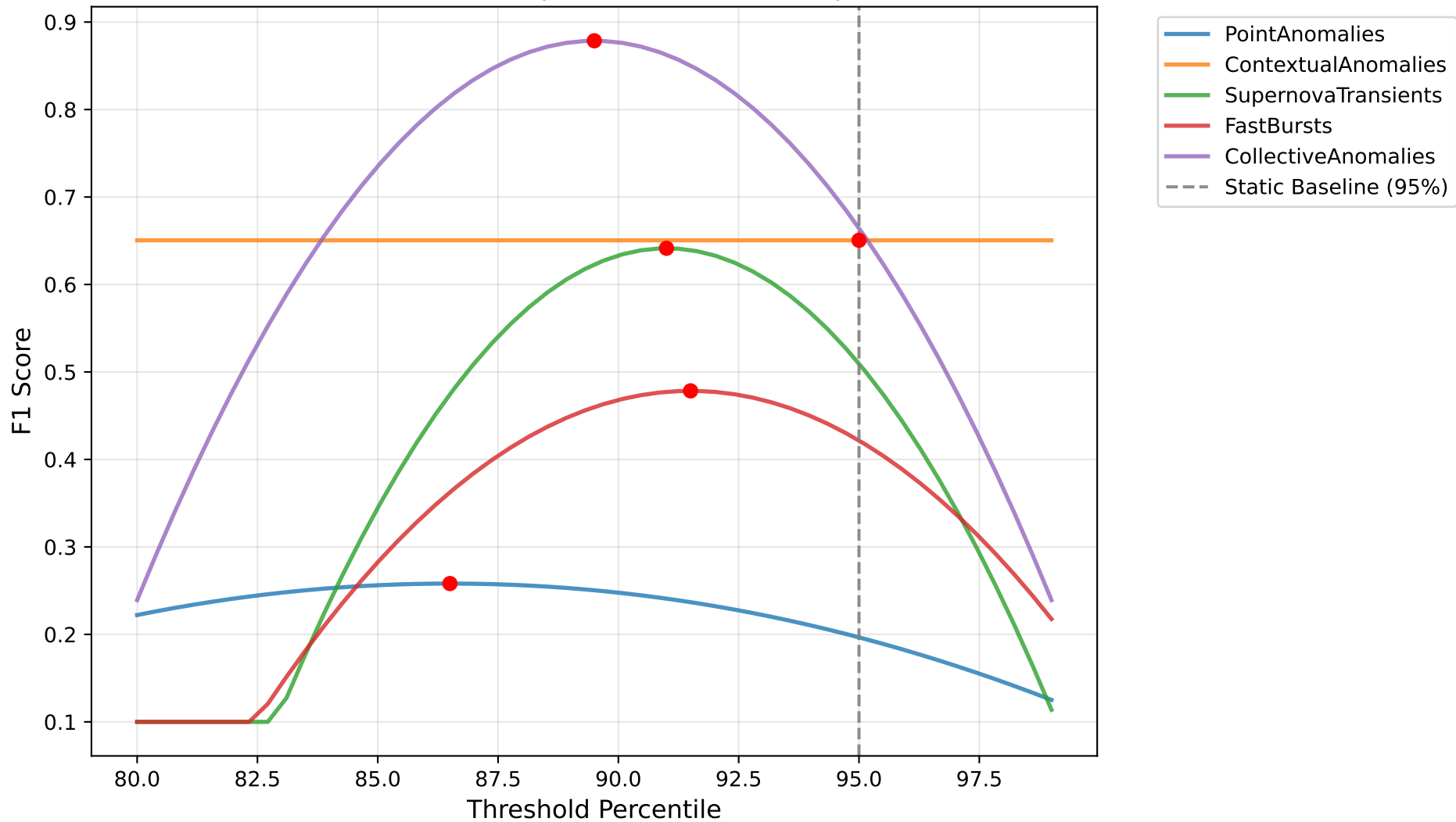
RL Threshold Optimization Landscape
