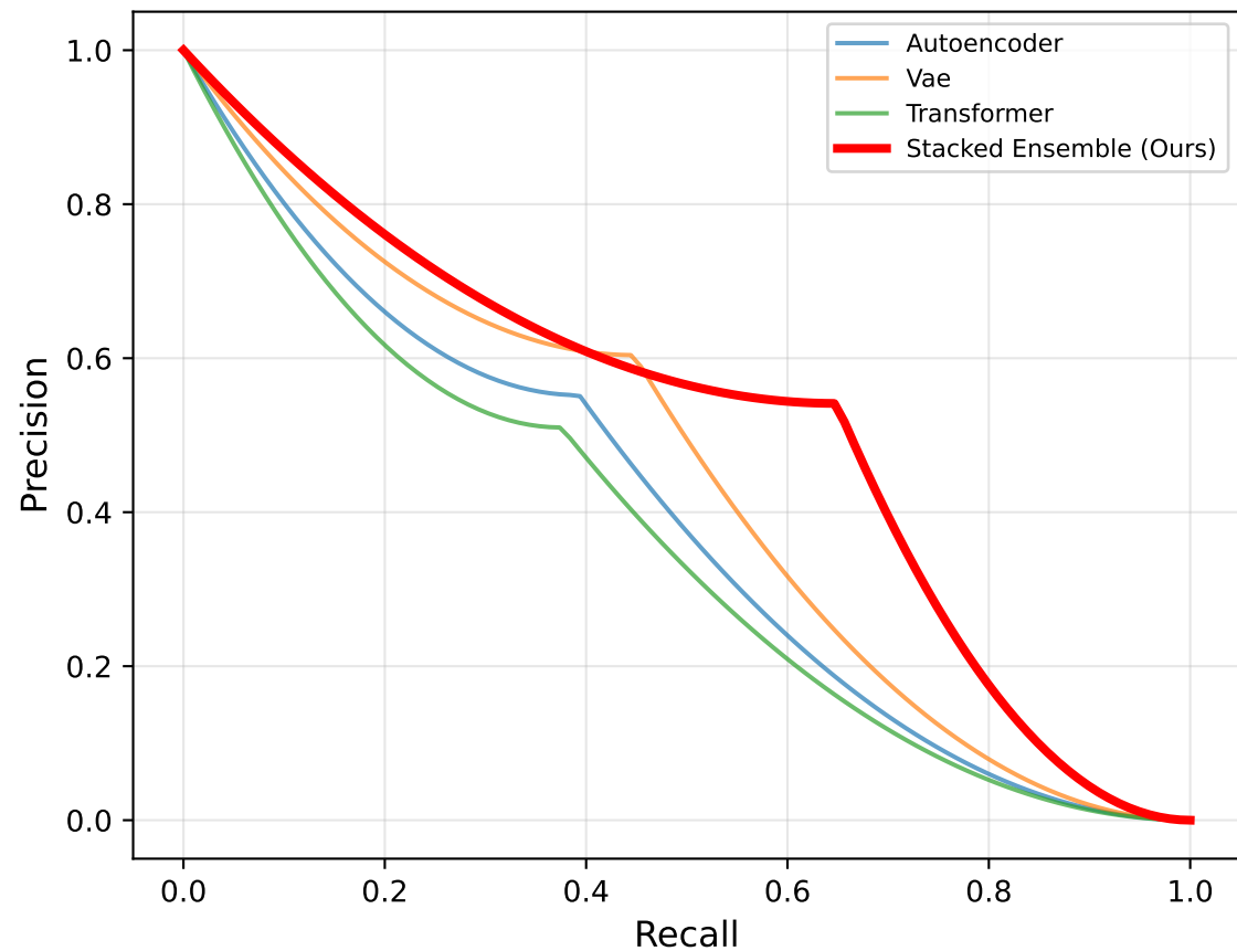
B: Mean Precision-Recall Curves
