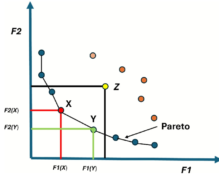
Figure 2.3: Example of a Pareto Front.[1]
