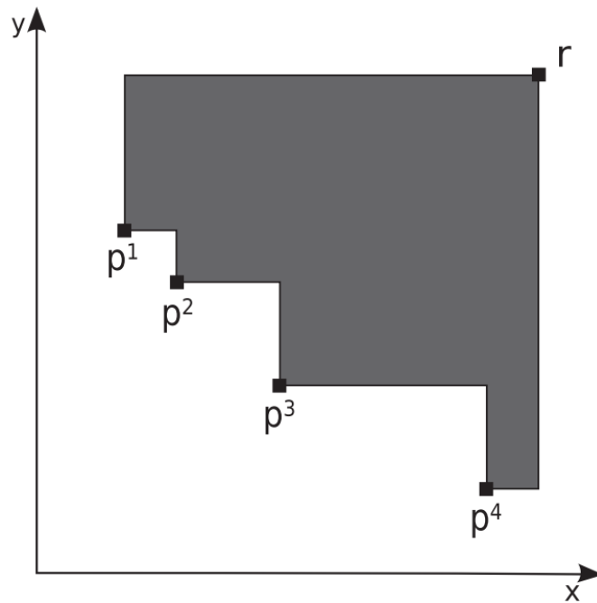
Figure 2.7: Hypervolume indicator [4].
