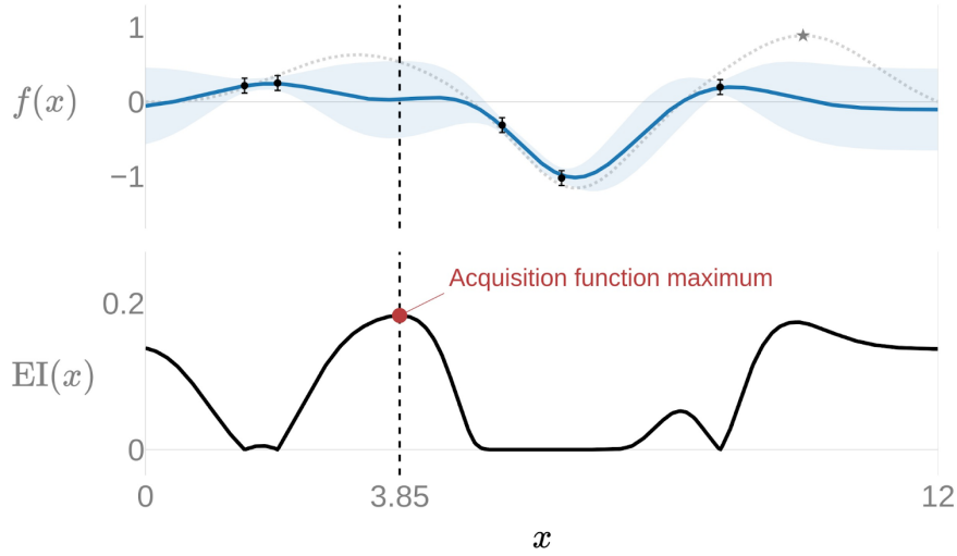
Figure 2.6: Acquisition Function [3].
