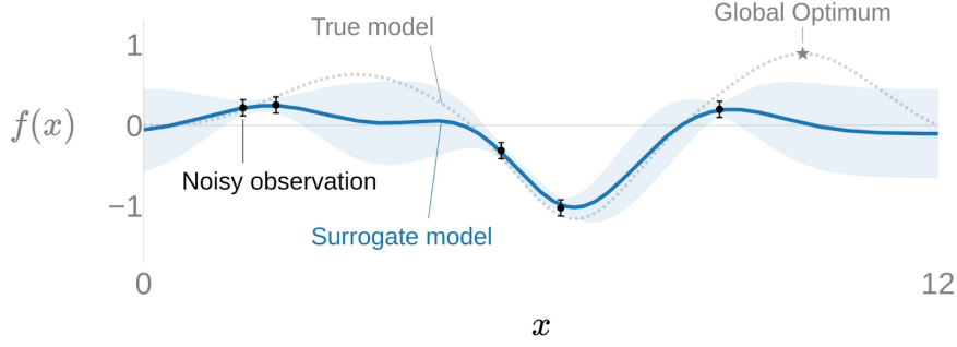
Figure 2.5: Surrogate Model [3].
