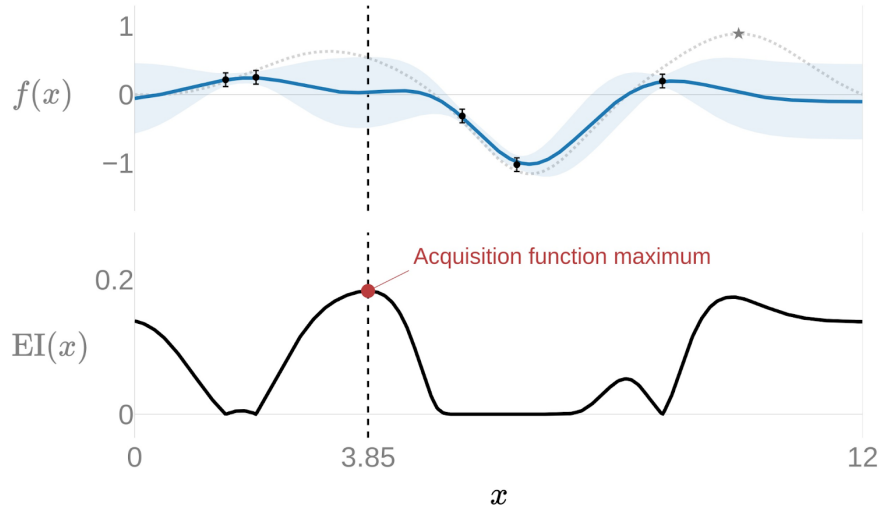
Figure 2.6: Acquisition Function [3].
