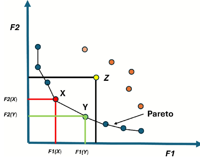
Figure 2.2: Example of a Pareto Front.[1]
