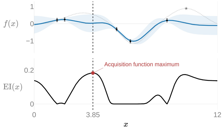
Figure 2.5: Acquisition Function [3].
