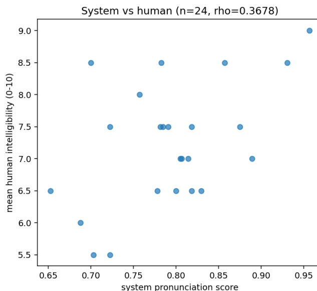
Figure 8.4: System pronunciation score against mean human intelligibility rating (0–10) across the 24 jointly-rated clips. Spearman’s \rho = 0.37 . The loose upward cloud reflects both a real positive association and the weak inter-rater agreement ( \alpha = 0.11 ) that bounds it.
