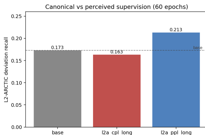
Figure 8.1: L2-ARCTIC deviation recall (60 epochs): baseline, the canonical-label adapter ( l2a_cpl_long ), and the perceived-label adapter ( l2a_ppl_long ). Canonical supervision falls below base ( 0.163 < 0.173 ); perceived supervision rises to 0.213. Same audio, opposite supervision target.
