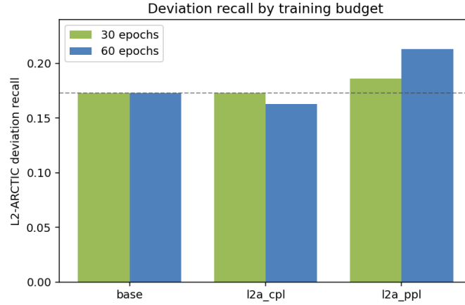
Figure 8.2: L2-ARCTIC deviation recall at 30 vs. 60 epochs. The canonical and perceived adapters separate further as the budget grows—canonical drifting down, perceived up—while the baseline (dashed) is unchanged.
