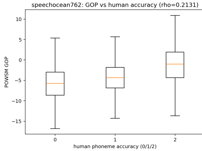
Figure 8.5: POWSM Goodness-of-Pronunciation against expert phoneme-accuracy labels on speechocean762 (2,500 utterances, 47,369 phones). Median GOP rises monotonically with the human accuracy score; phone-level Spearman’s \rho = 0.21 .
