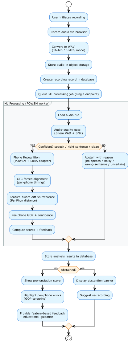
Figure 6.2: Activity Diagram: Pronunciation Assessment Workflow
