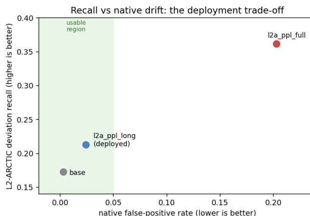
Figure 8.6: Deviation recall against native false-positive rate for the baseline, the deployed 12a_pp1_long , and the full-corpus 12a_pp1_full . The shaded band marks a usable native-drift budget (FPR < 0.05); the highest-recall adapter falls far outside it, which is why the deployed model is the more conservative 12a_pp1_long .
