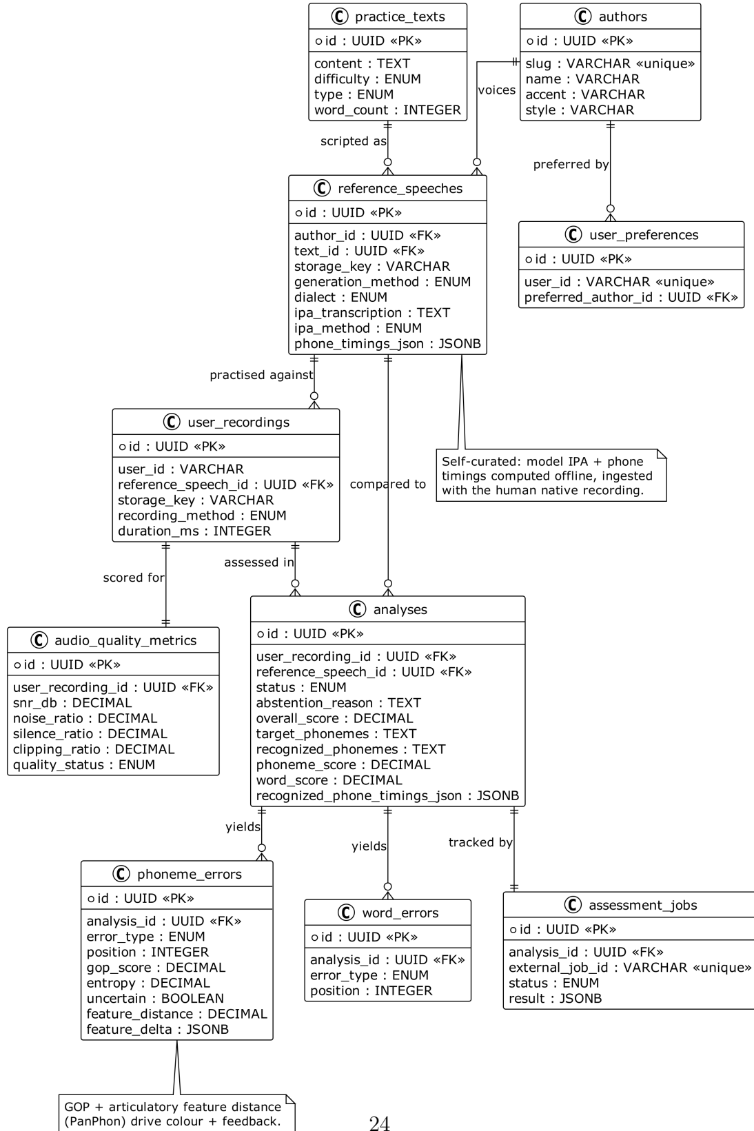
Figure 6.1: Entity-Relationship Diagram for Nounce
